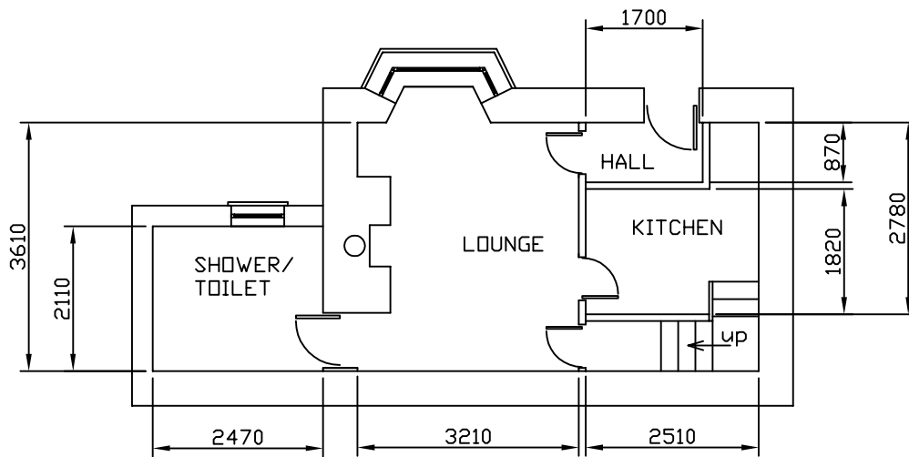
GROUND FLOOR AREA = 28 SQUARE METERS
