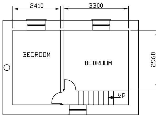
1ST FLOOR AREA = 22 SQUARE METERS
