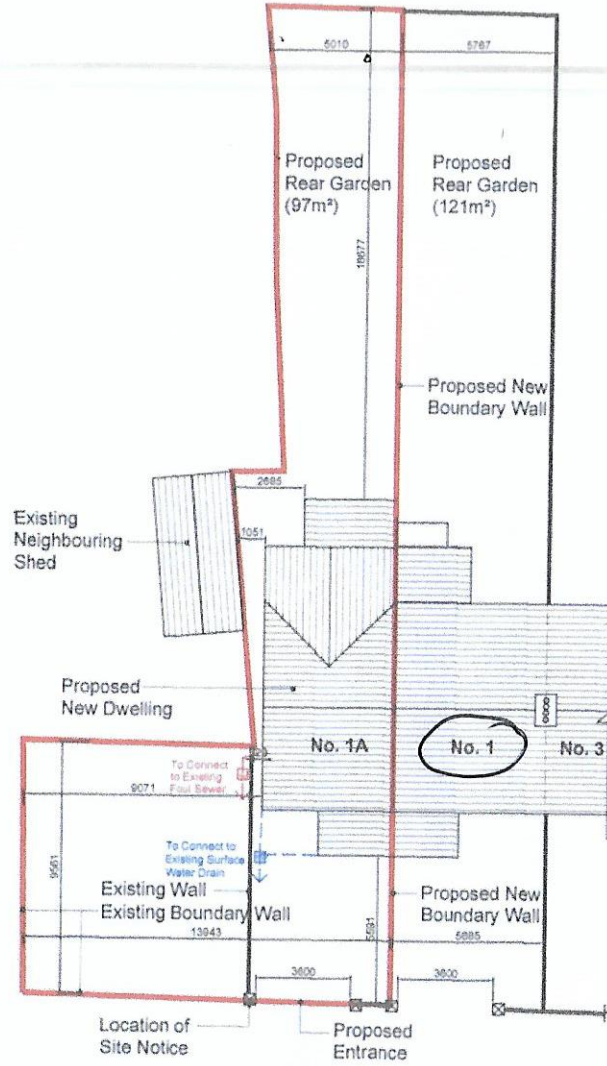
PROPOSED SITE PLAN Scale: 1:200 Area: 0.0684 Ha
