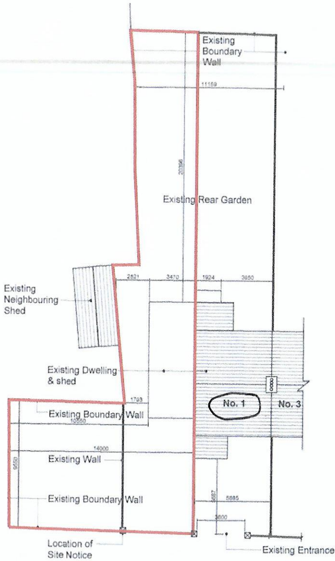
EXISTING SITE PLAN SCALE 1:200
