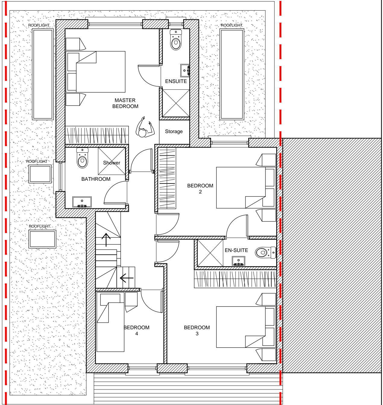
PROPOSED FIRST FLOOR PLAN ....NOT TO SCALE OPTION 1 - 60 Sq Metres
