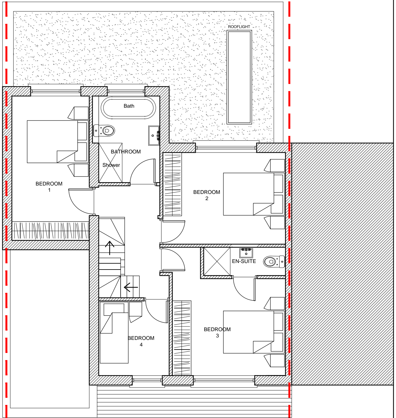
PROPOSED FIRST FLOOR PLAN ....NOT TO SCALE OPTION 2 - 58 Sq Metres
