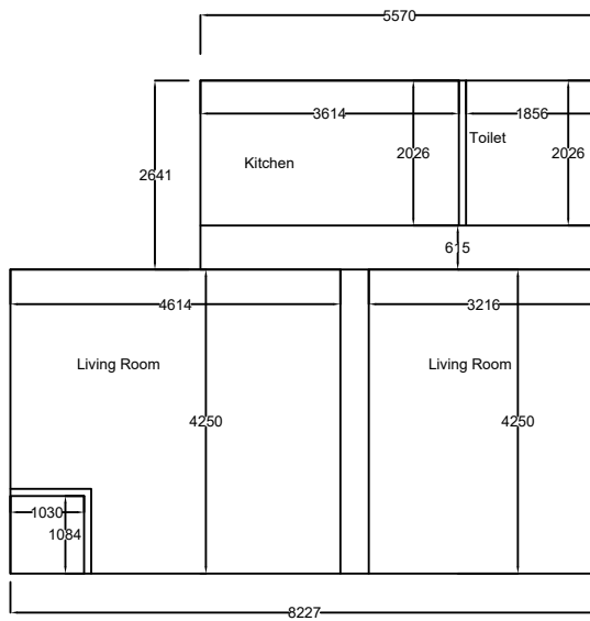
Ground Floor Area = 49.68m2
