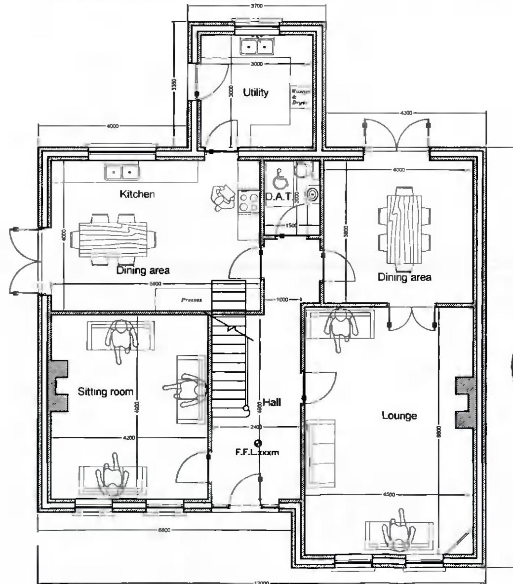
PROPOSED GROUND FLOOR PLAN (Area 118.5m 2 - 1276ft 2 )
