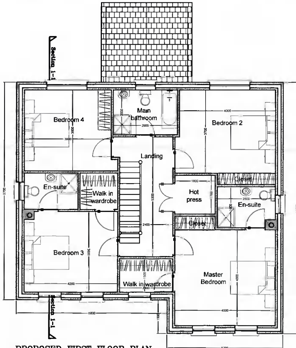
PROPOSED FIRST FLOOR PLAN (Area 108.45m 2 - 1167ft 2 )
