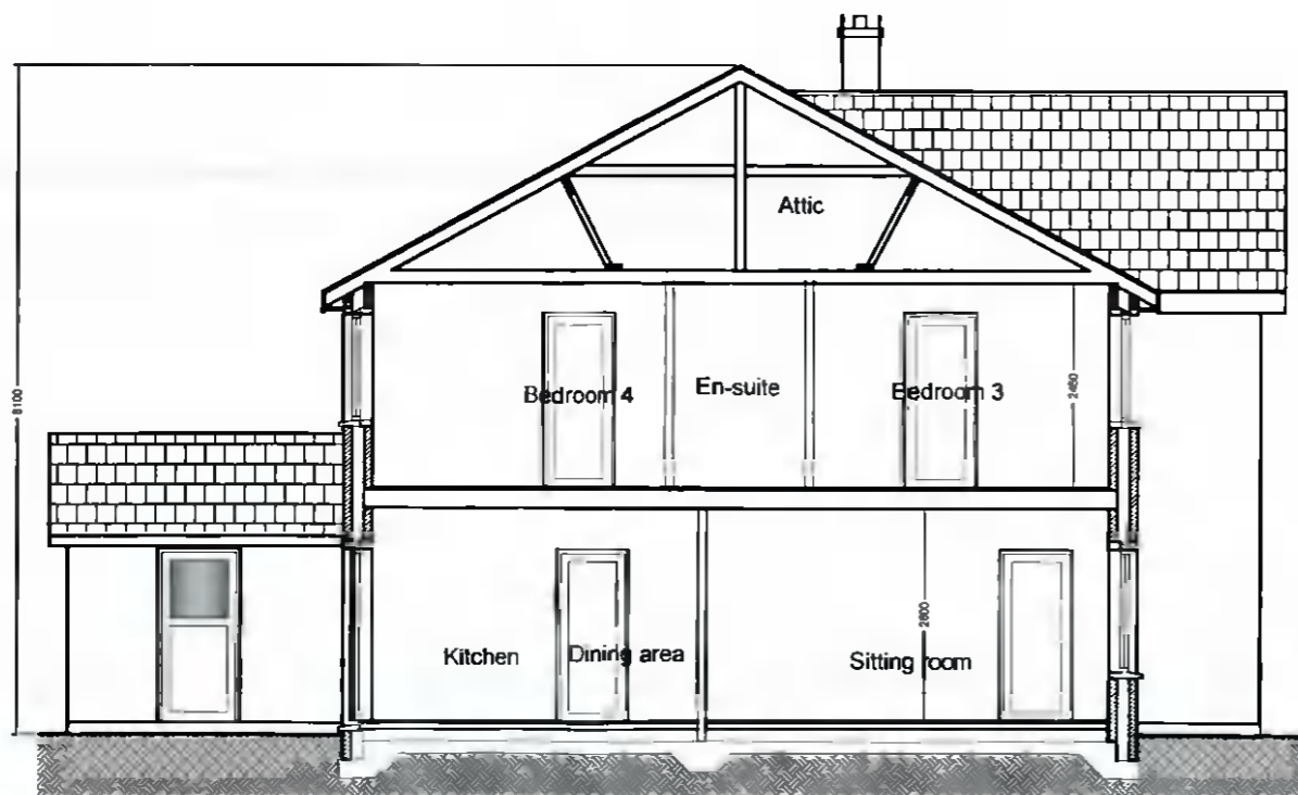
EXISTING SECTION 1-1
