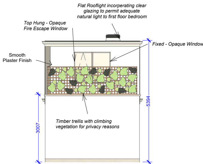
Rear Elevations
