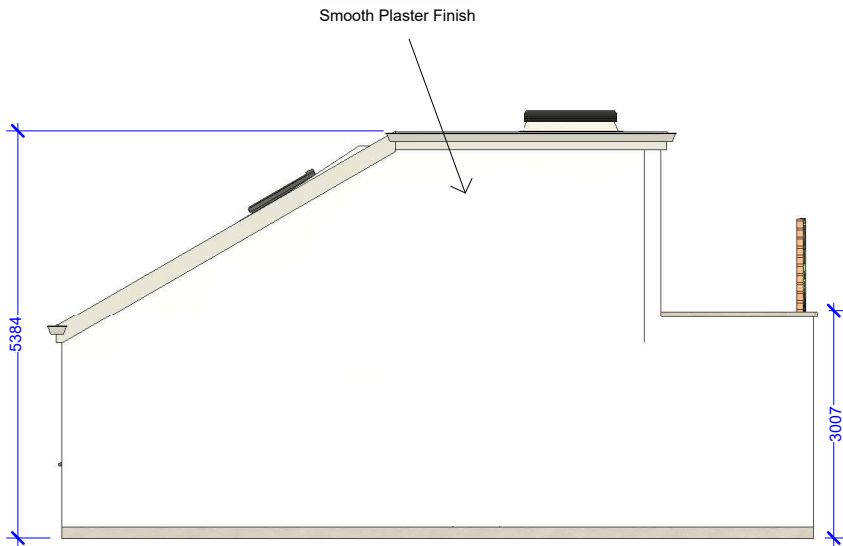
Left Elevations
