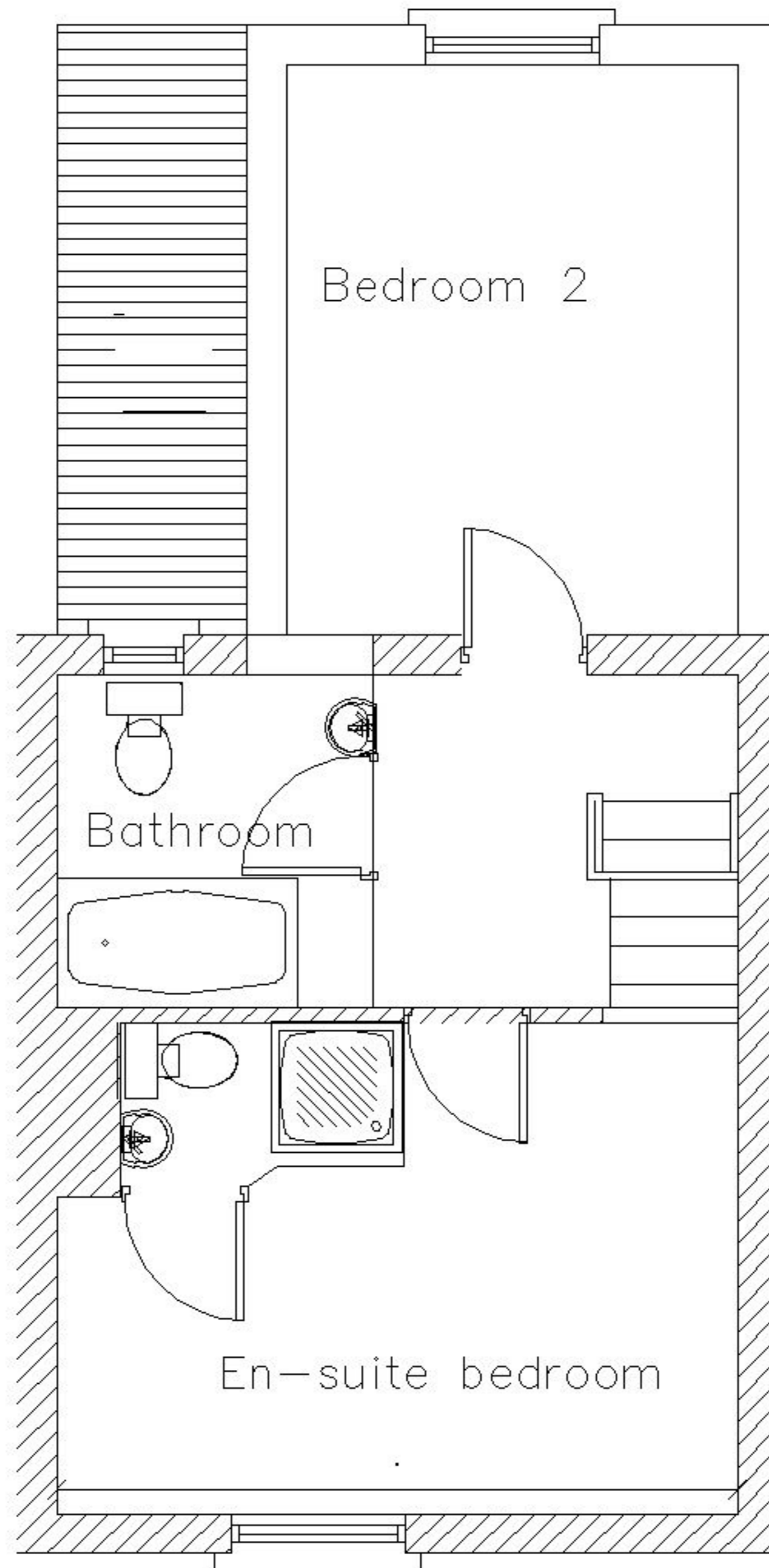
FIRST FLOOR
