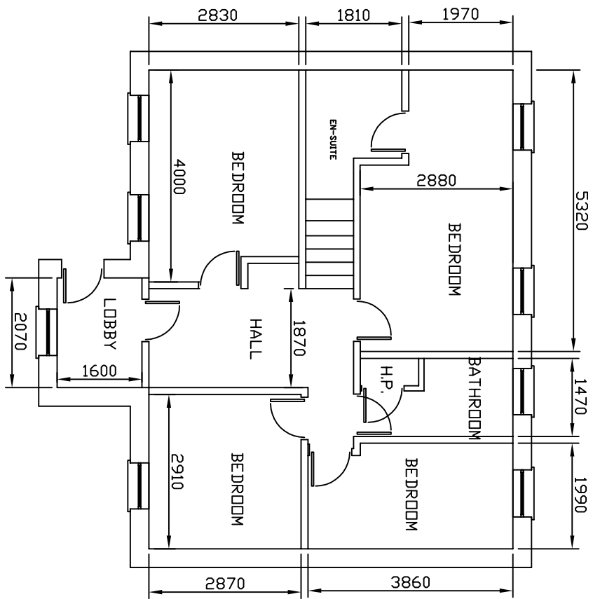
GROUND FLOOR PLAN - FLOOR AREA: 65.5 SQ. MTRS.
