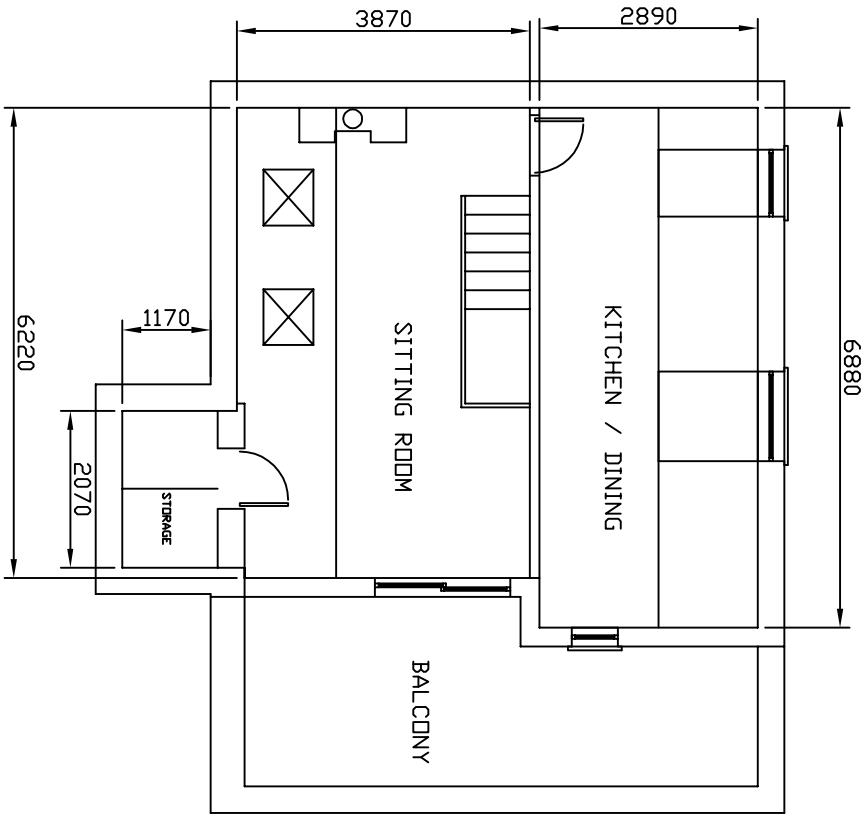
1ST FLOOR PLAN - FLOOR AREA: 48 SQ. MTRS
