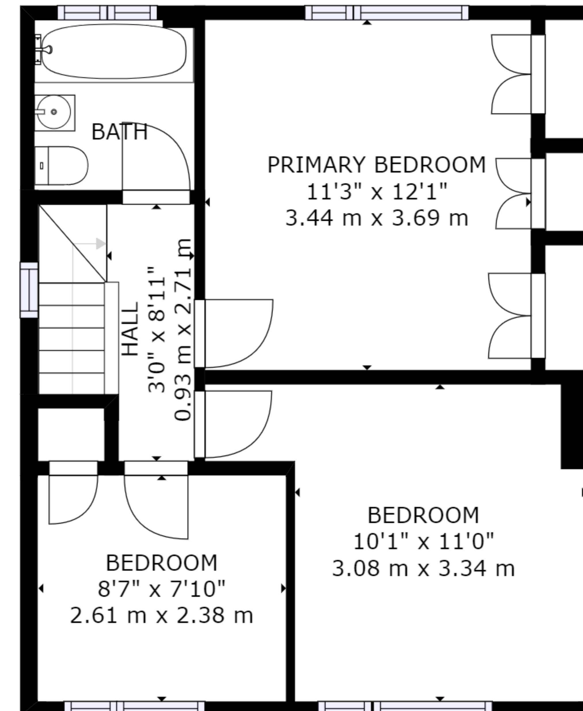
FLOOR 2
