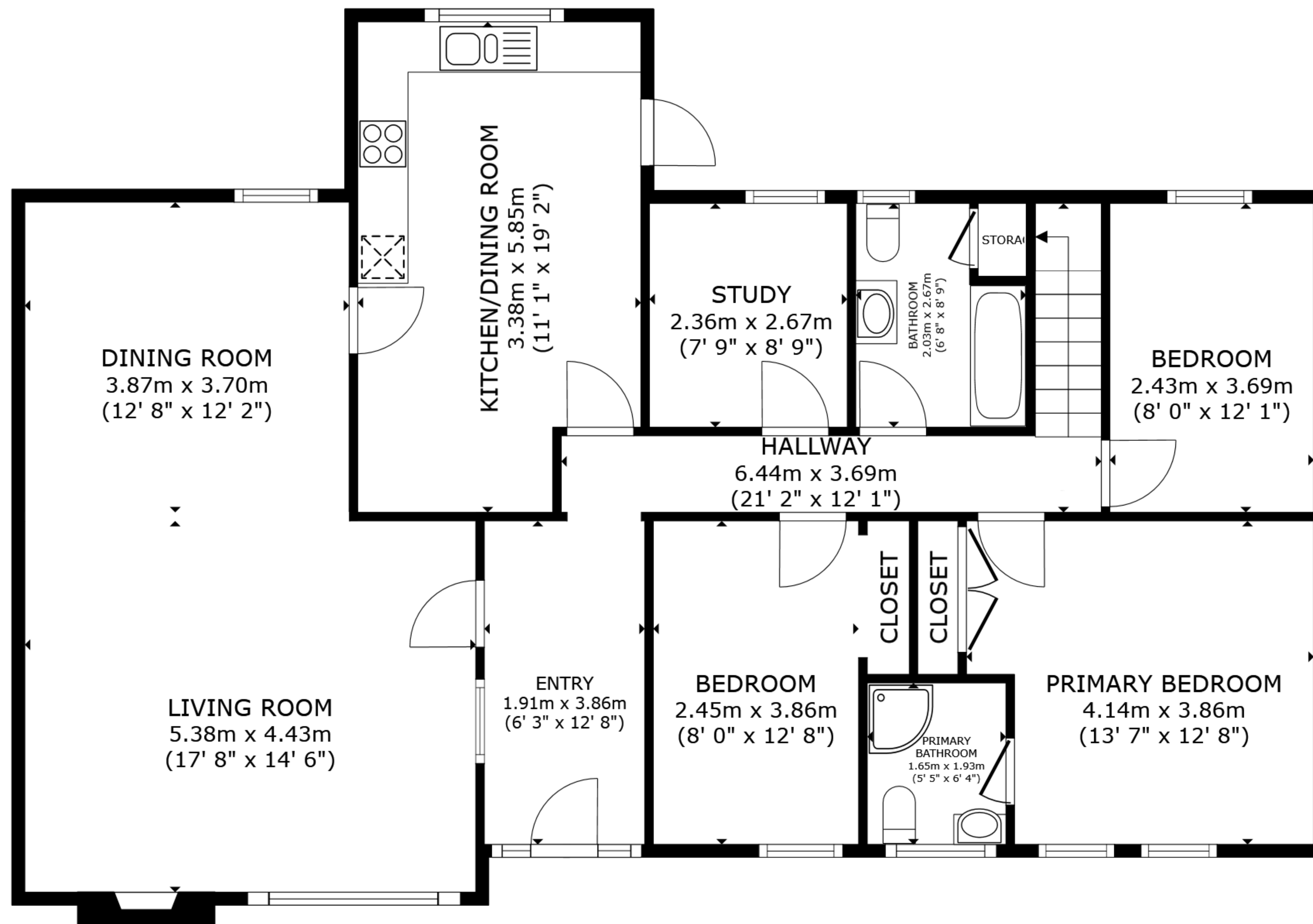
FLOOR 1
