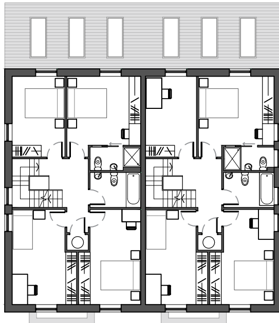
FIRST FLOOR TYPE A
