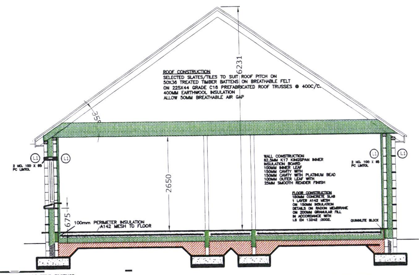
Section Y-Y
