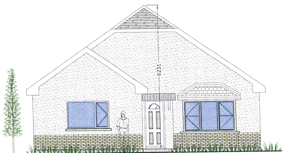
EAST ELEVATION
