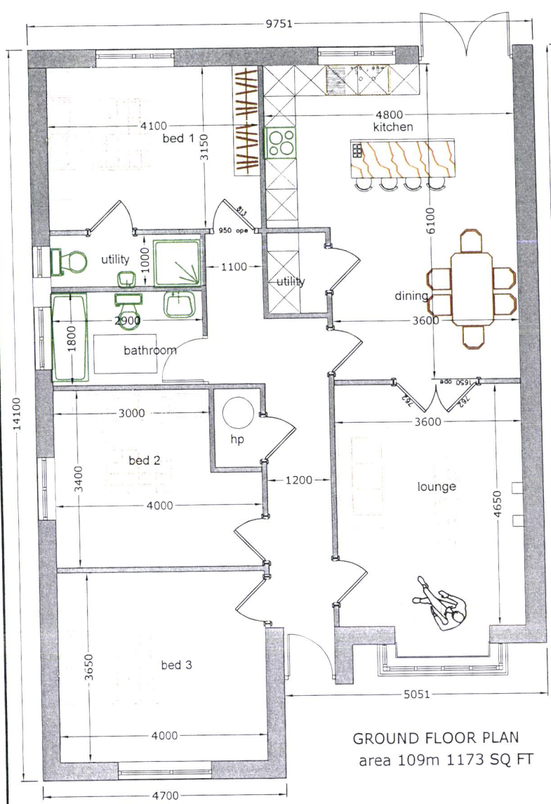
Floor plan
