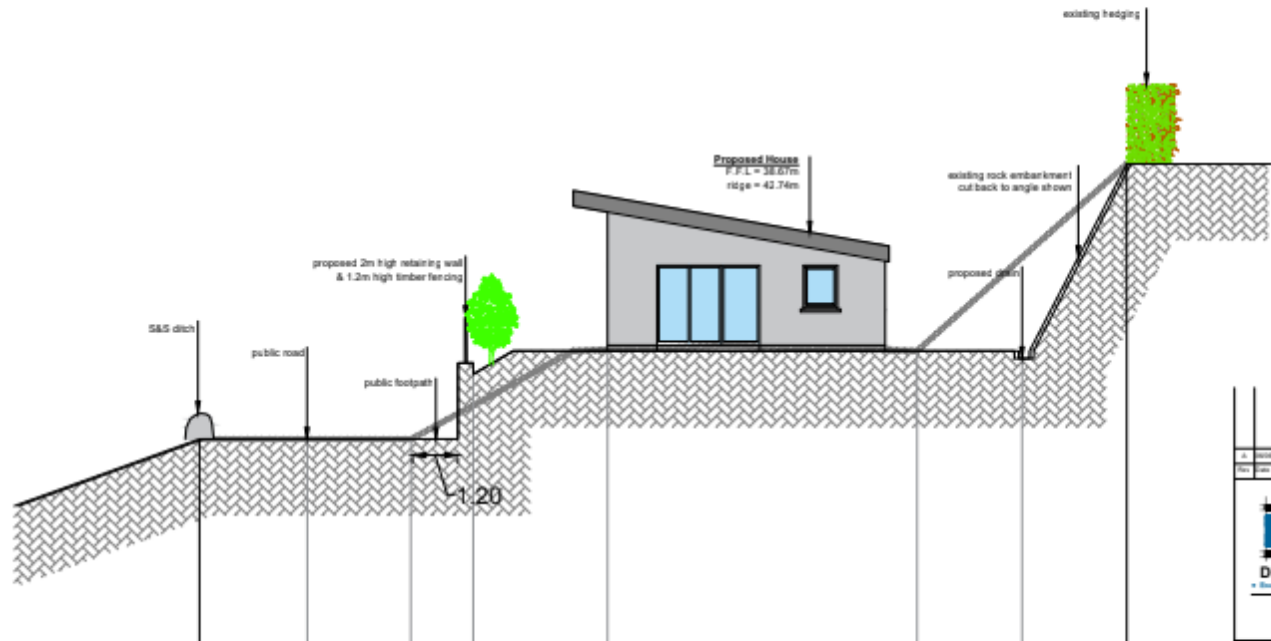
Site Section Z-Z
