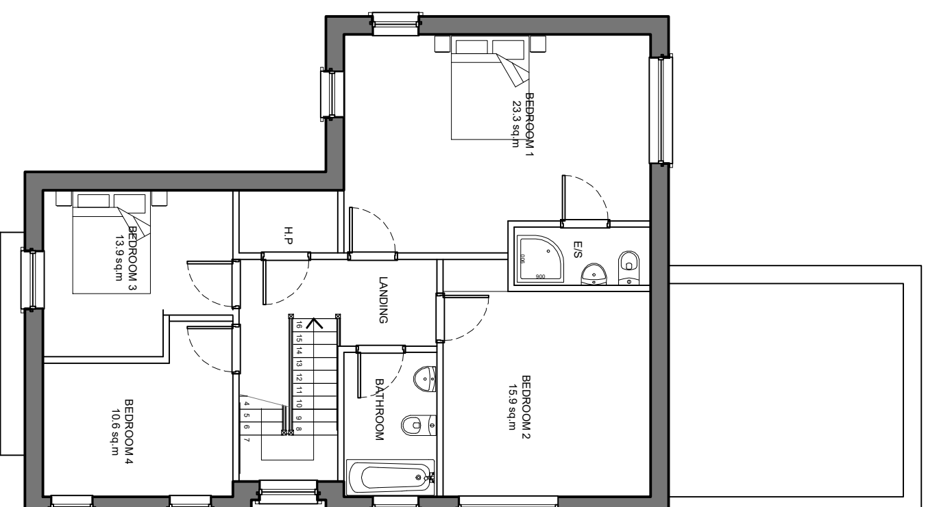
SITE 5 FIRST FLOOR PLAN FF AREA = 86.7m 2 , (O/A 933ft 2 )
