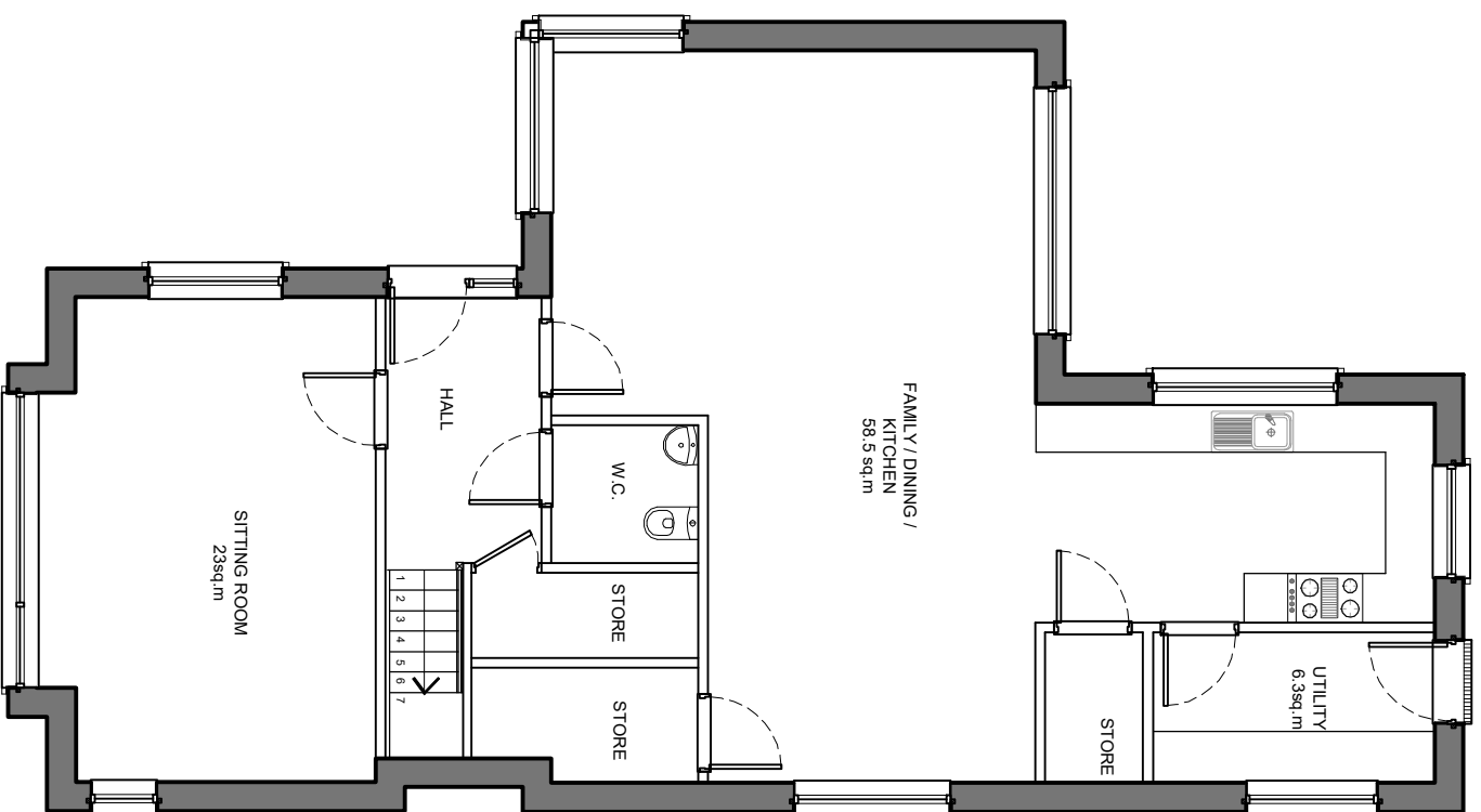
SITE 5 GROUND FLOOR PLAN GF AREA = 110.8m 2 , (O/A 1193ft 2 )
