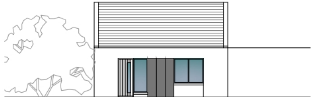
NORTH ELEVATION (Wolfetone St) SCALE=1:100
