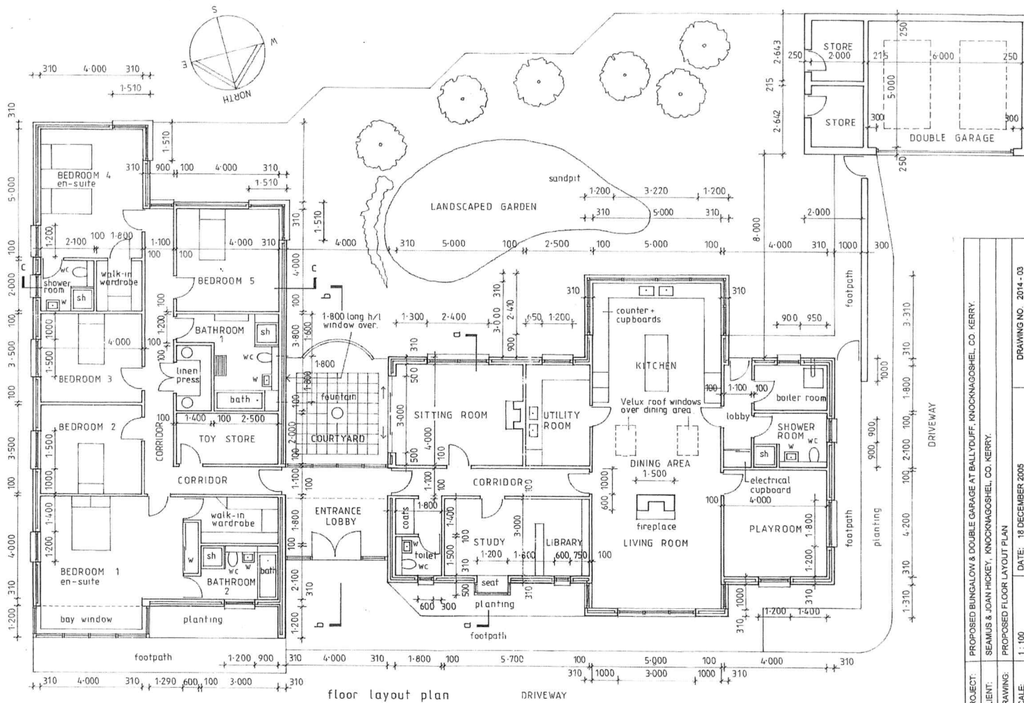
floor layout plan
