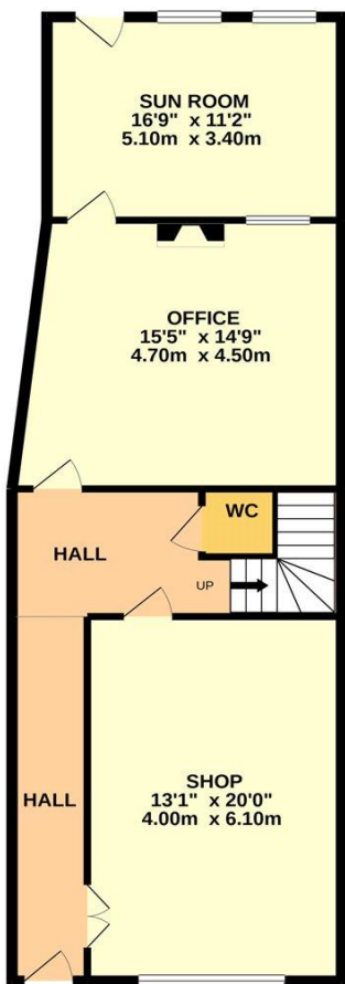
GROUND FLOOR 862 sq.ft. (80.1 sq.m.) approx.
