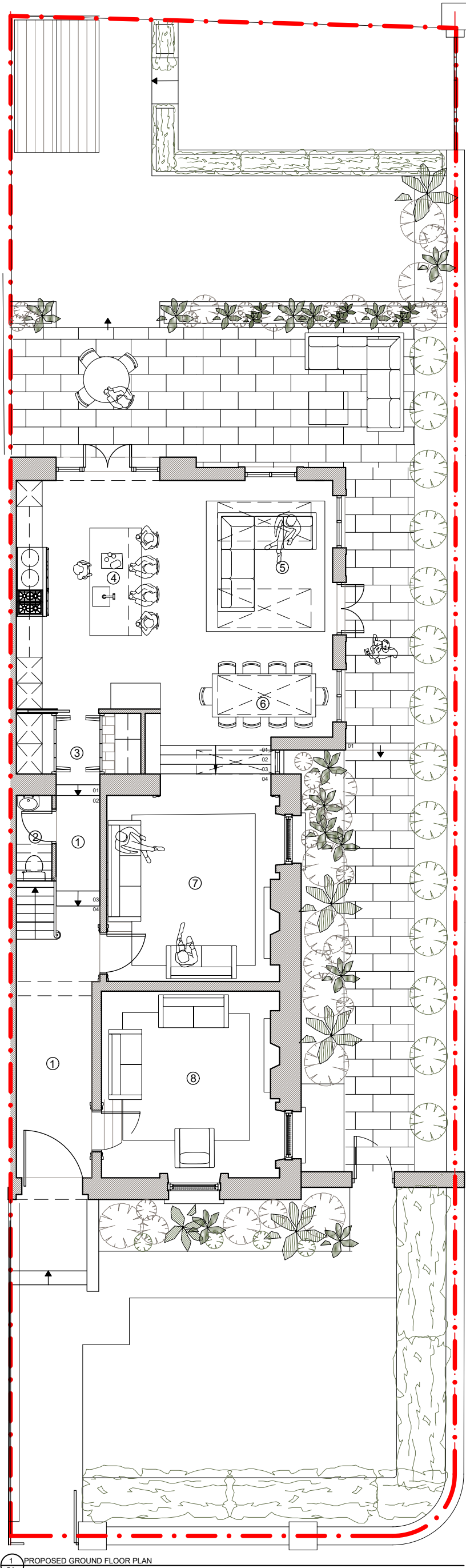
1 PROPOSED GROUND FLOOR PLAN
