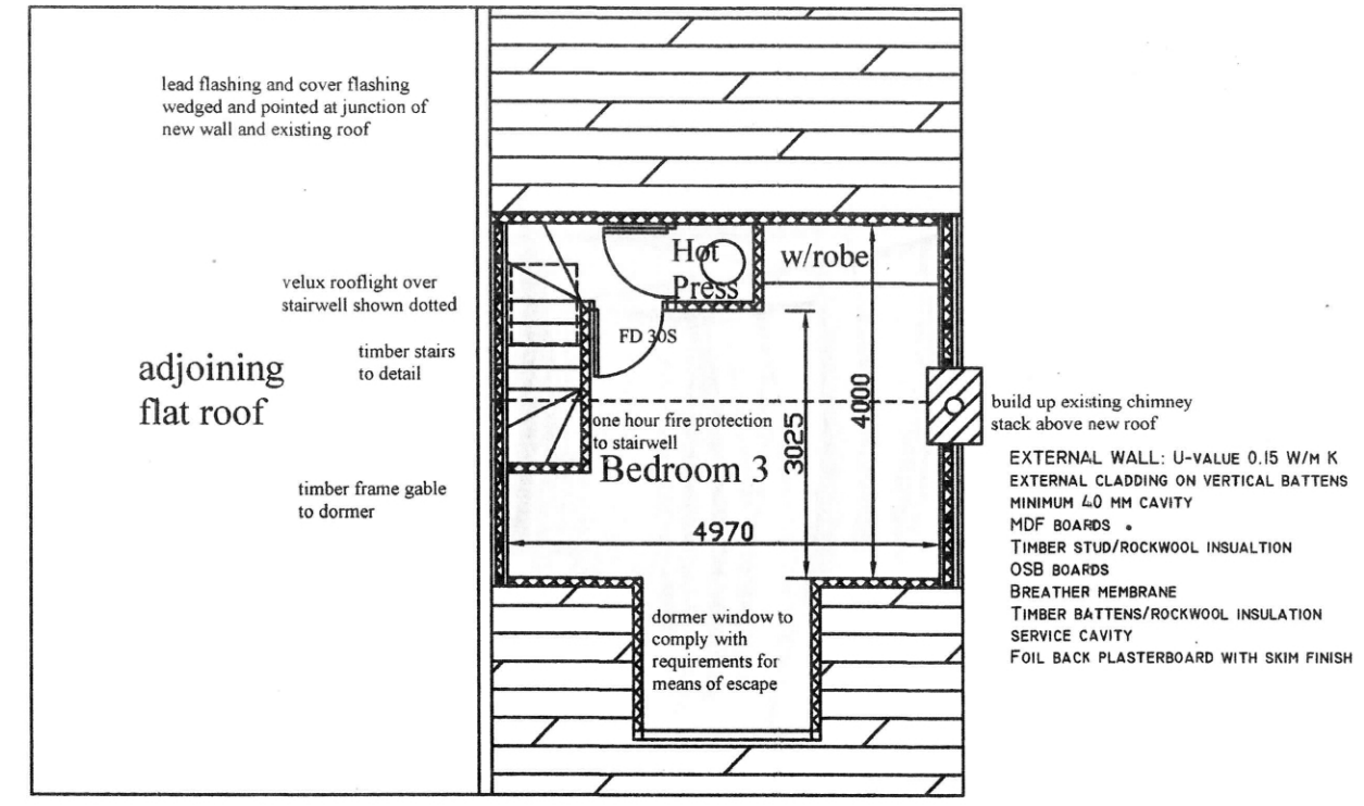
ROOF SPACE FLOOR PLAN
