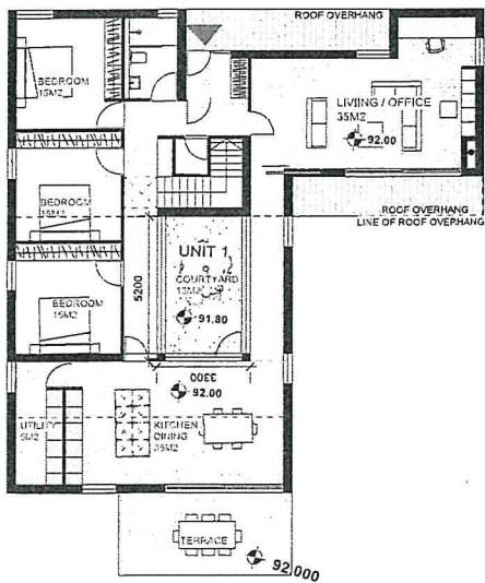
UNIT 1 - GROUND FLOOR PLAN SCALE 1.200 A4
