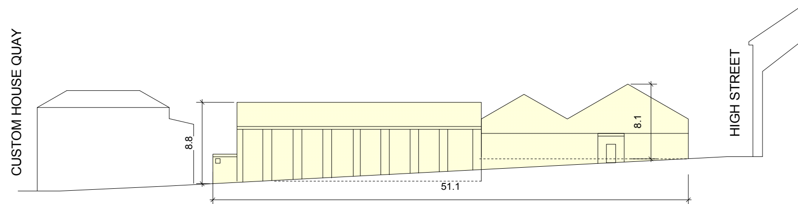
SIDE ELEVATION OF EXISTING BUILDINGS
