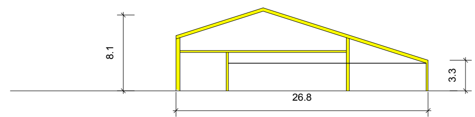
CROSS SECTION OF EXISTING BUILDING
