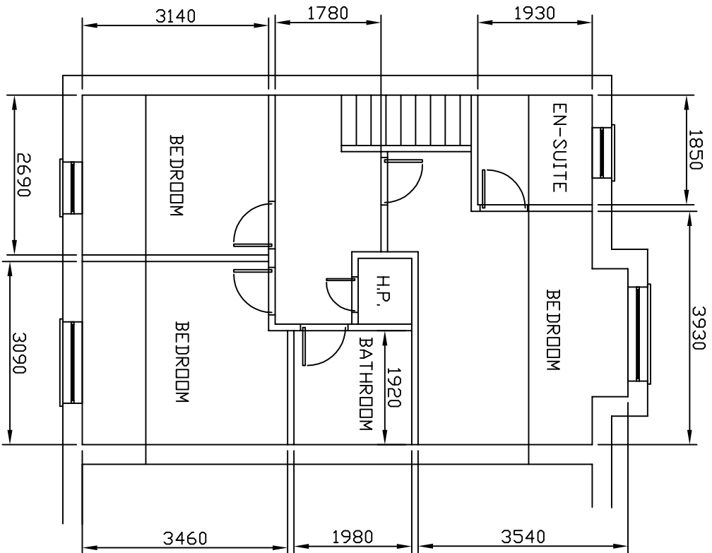
FIRST FLOOR AREA = 52 SQUARE METERS
