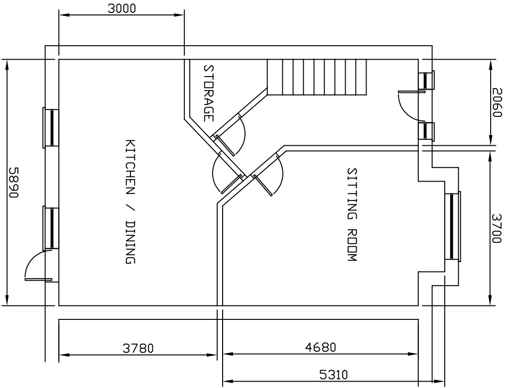
GROUND FLOOR AREA = 52 SQUARE METERS
