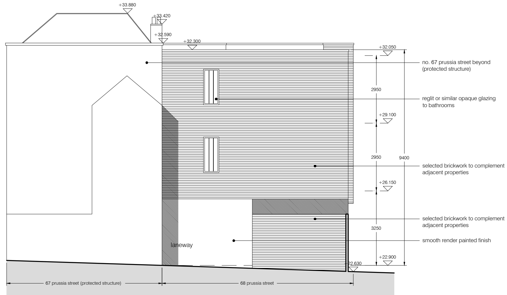
PROPOSED ELEVATION TO REAR LANEWAY
