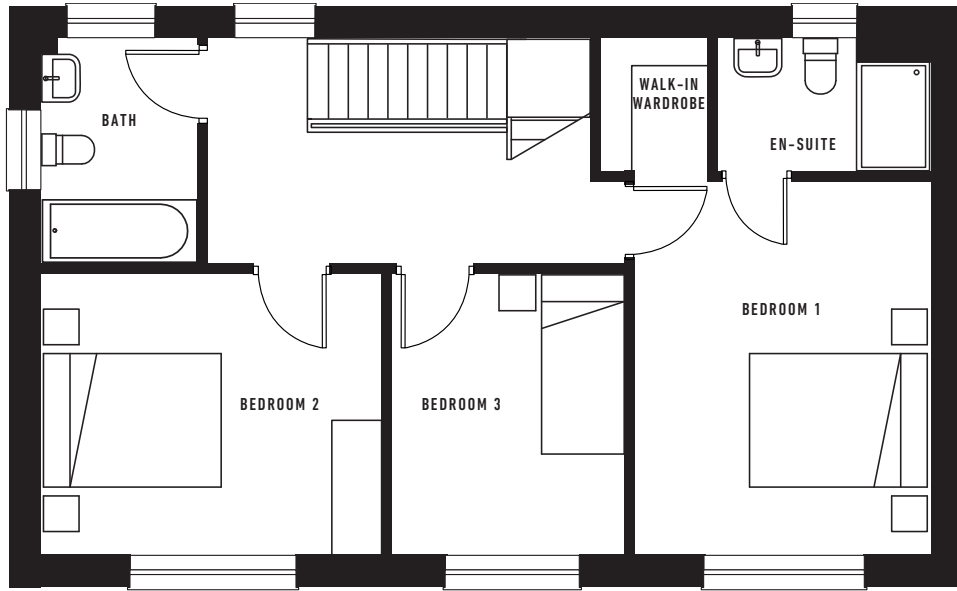
FIRST FLOOR
