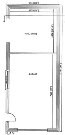
PLAN
