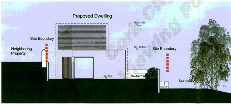
1 pl-200 Proposed Section B-B Scale 1:125
