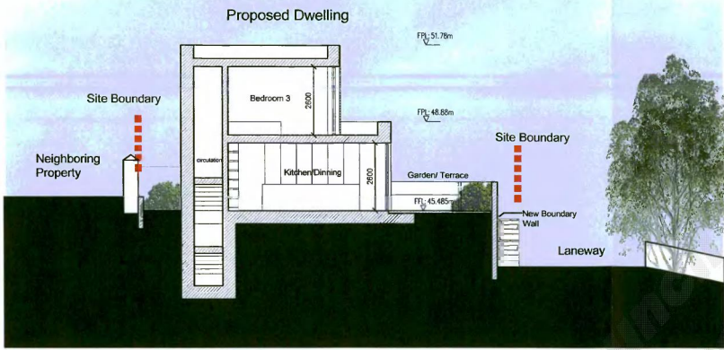
1 pl-200 Proposed Section B-B Scale 1:125
