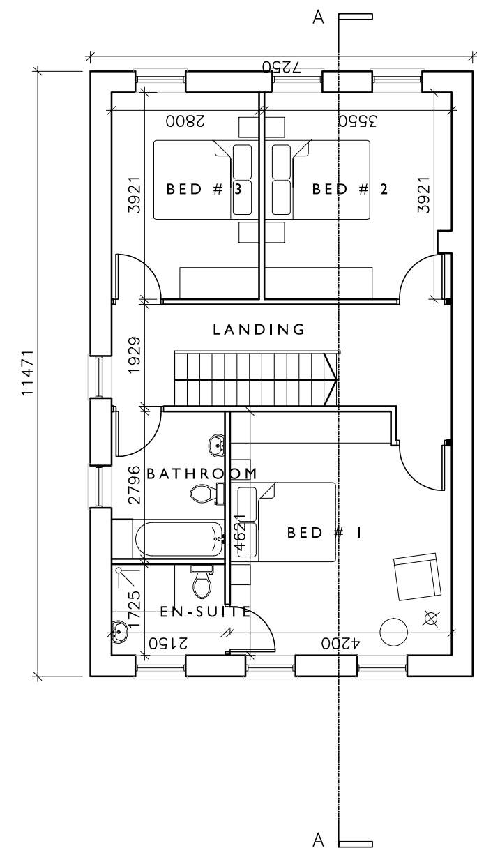
02 202 PROPOSED FIRST FLOOR PLAN 1:100
