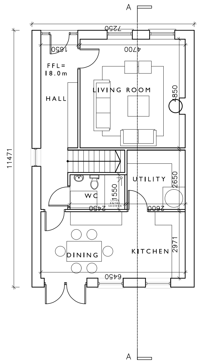
01 202 PROPOSED GROUND FLOOR PLAN 1:100
