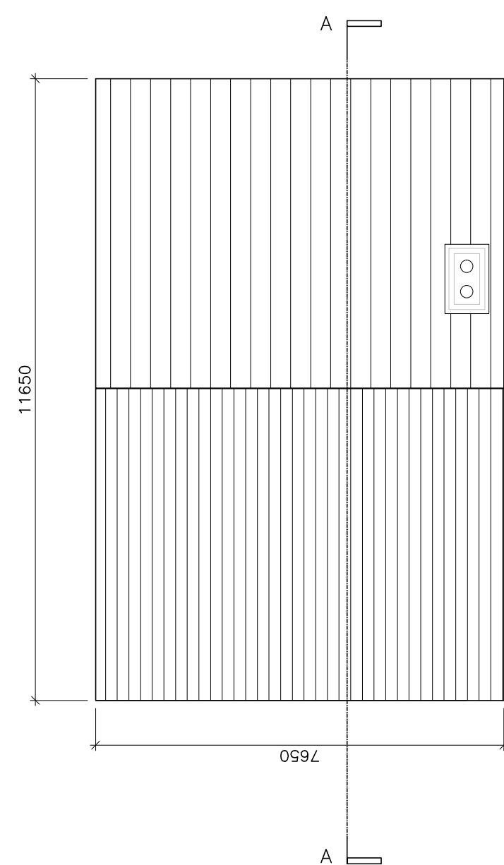
03 202 PROPOSED ROOF PLAN 1:100
