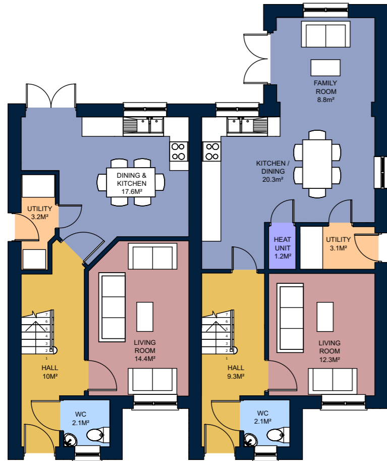
HOUSE TYPE E GROUND FLOOR
