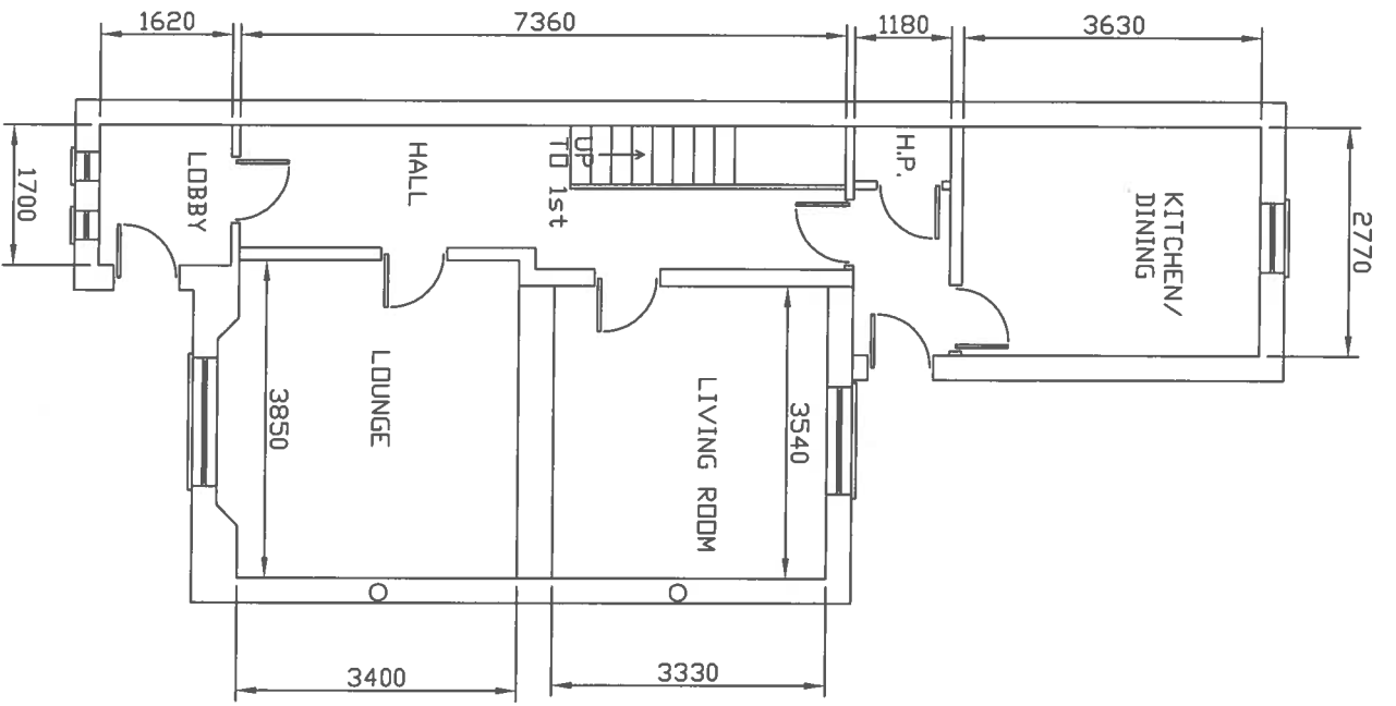
Ground Floor Total Approximate Area - 58 sqm
