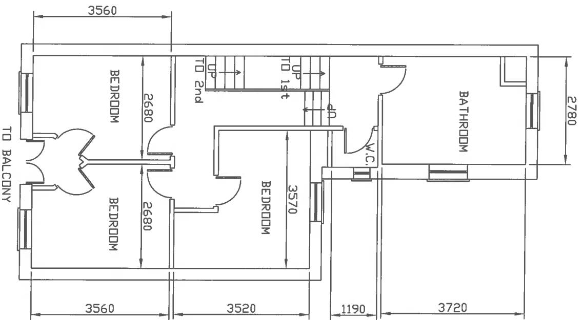
First Floor Total Approximate Area - 55 sqm
