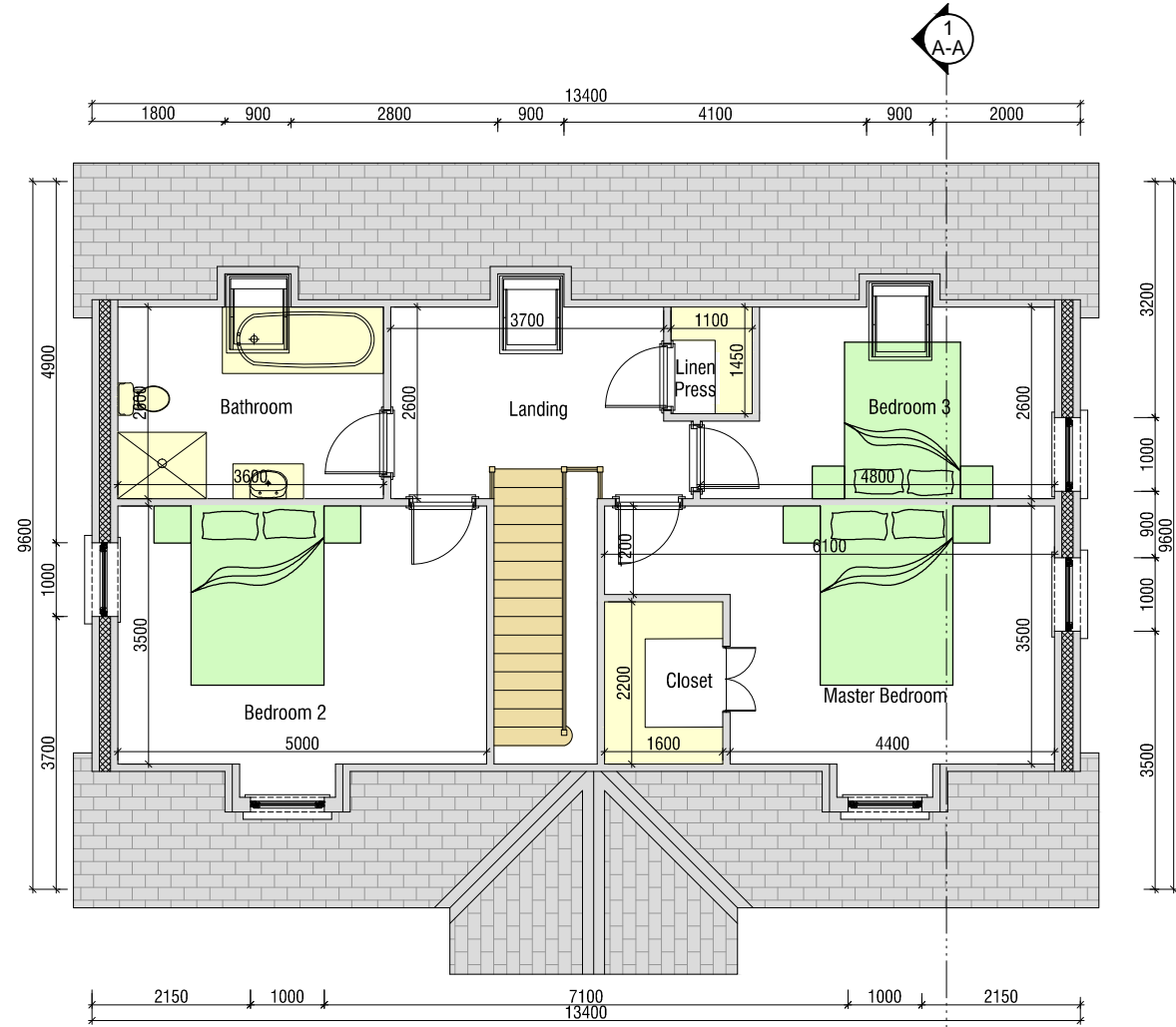
Dwelling First Floor Plan Scale 1-100
