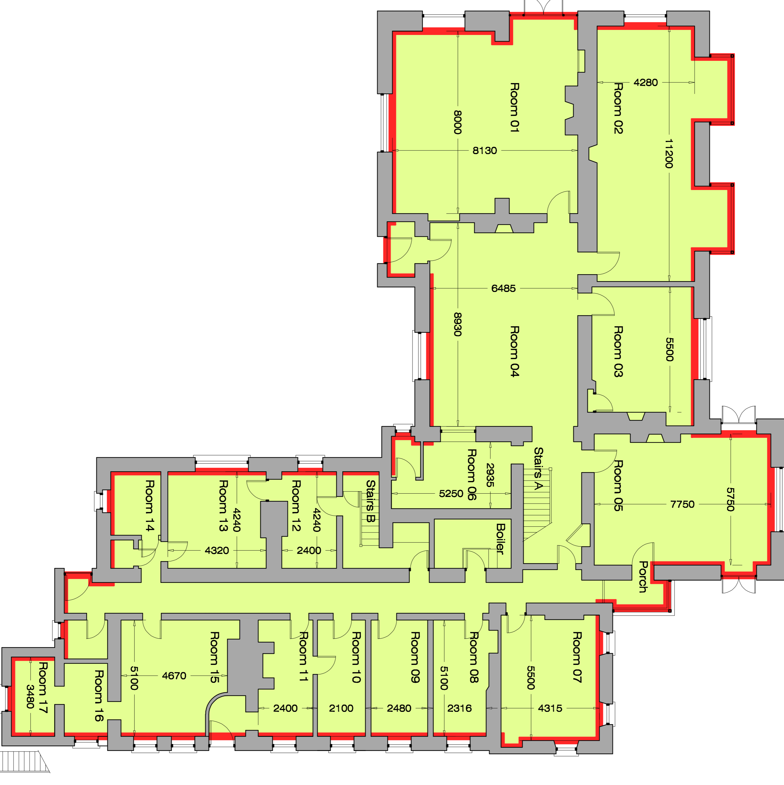
GROUND FLOOR Floor area 564sqm
