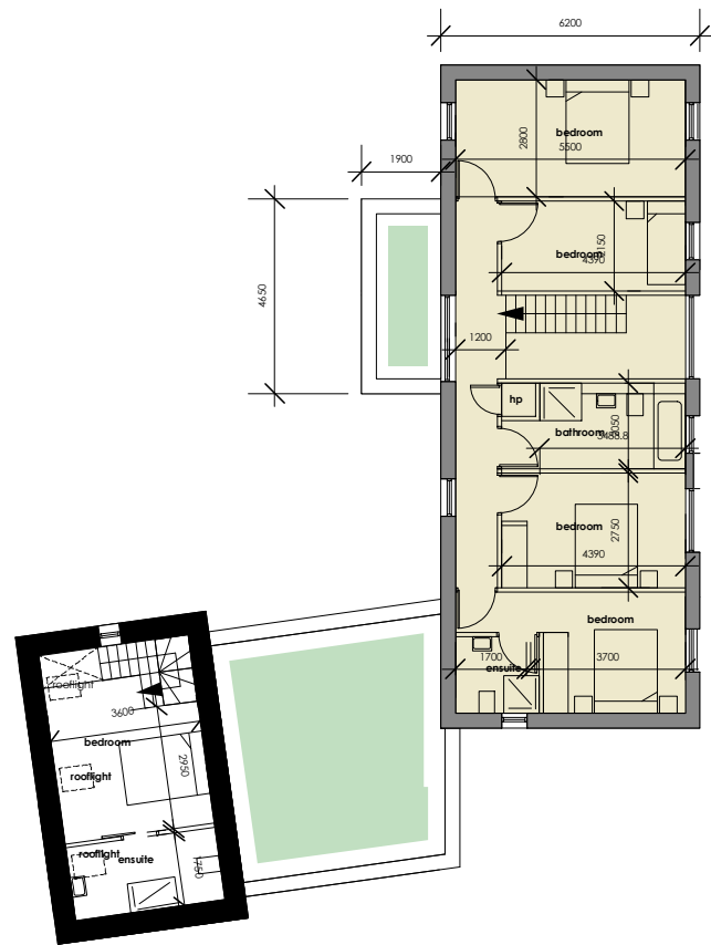
first floor plan (existing 22m2, proposed 80m2)
