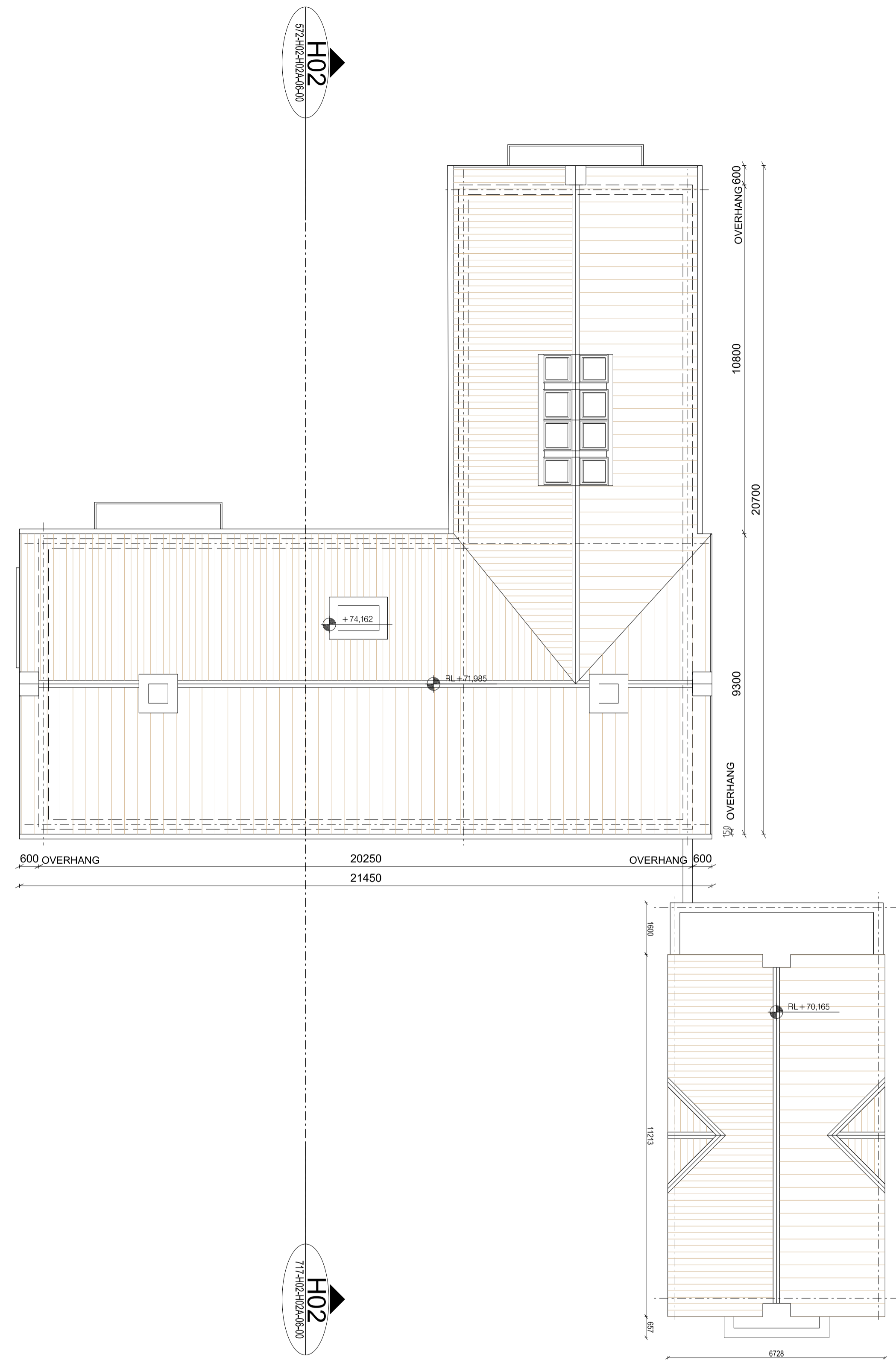
1 ROOF PLAN 1:100
