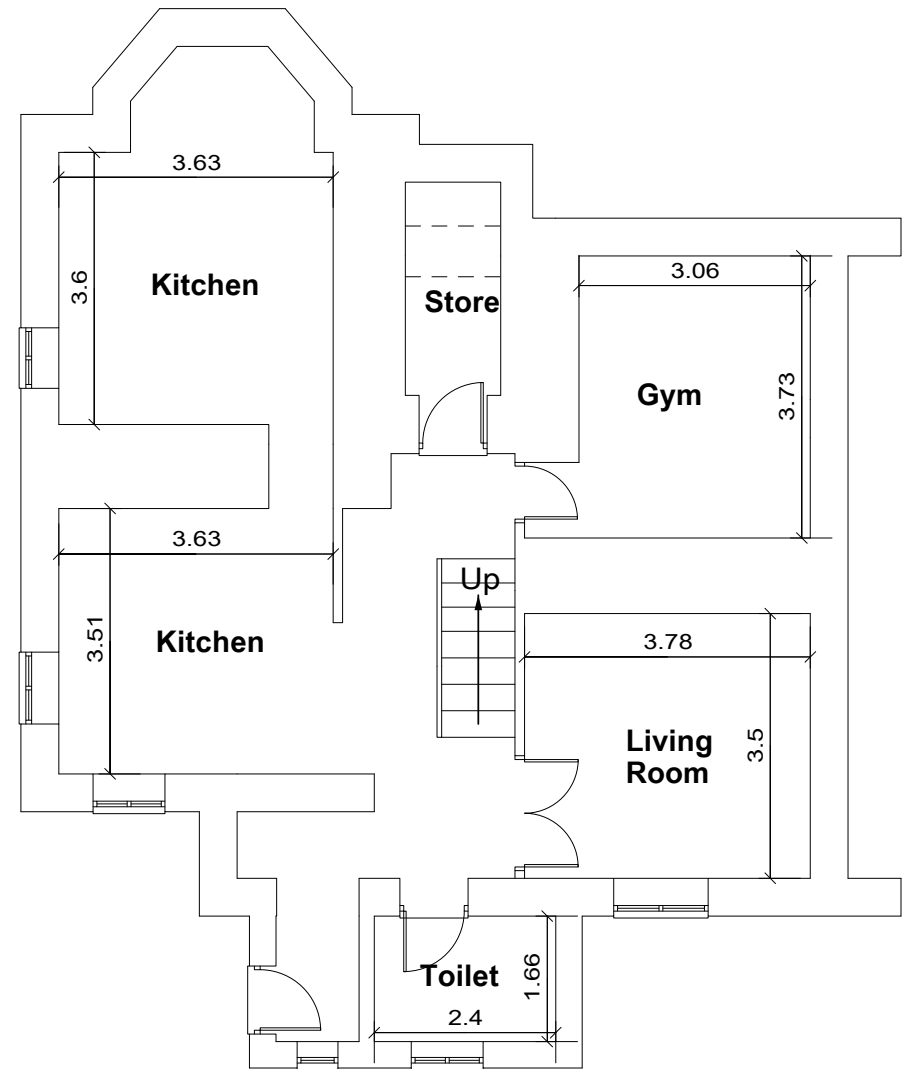
ENTRANCE LEVEL - 1 (Area 96.6m 2 )
