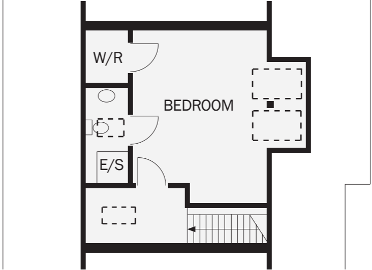
LEVEL 2 PLAN
