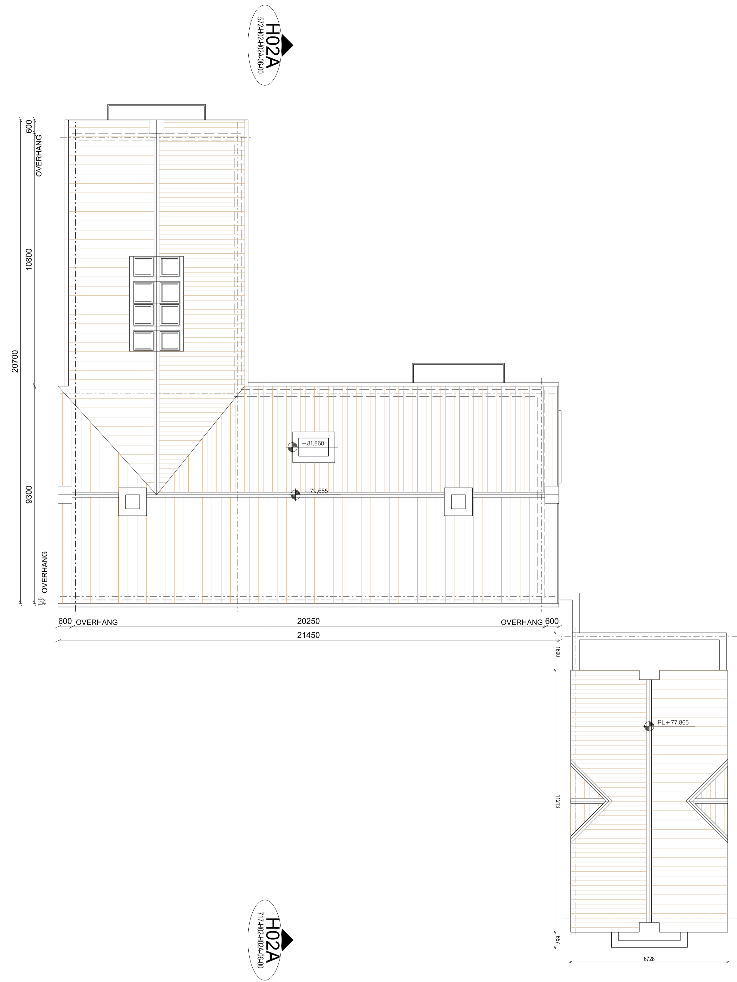
1 ROOF PLAN 1:100
