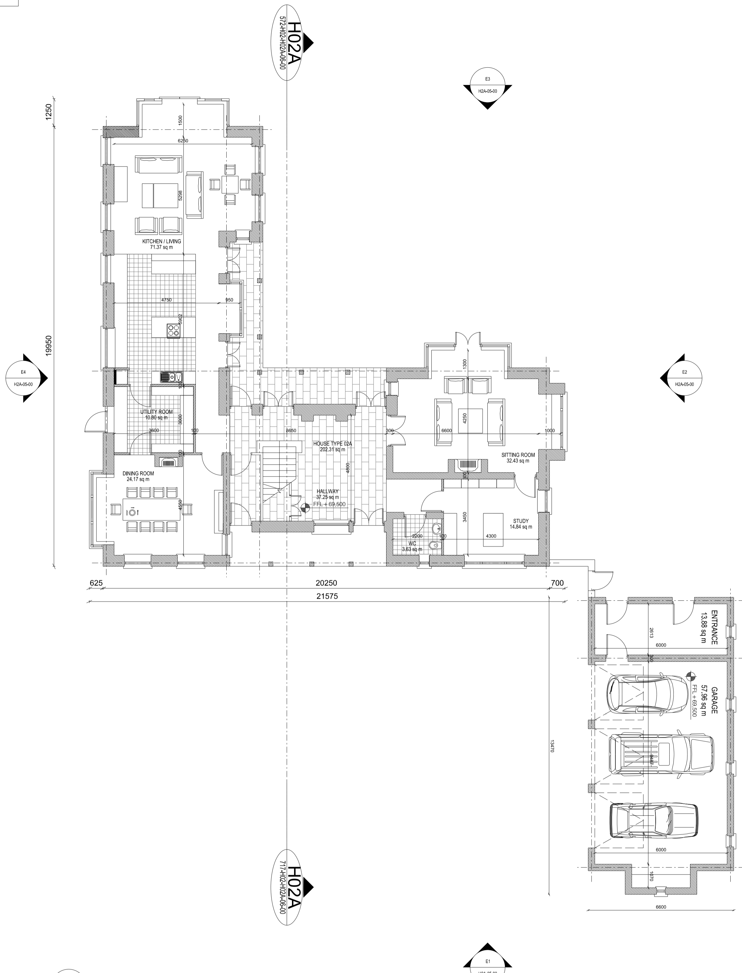
1 GROUND FLOOR PLAN 1:100
