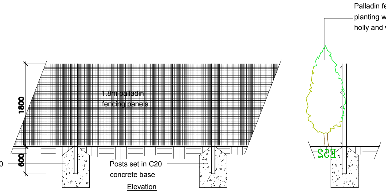
Palladin Fencing Detail Scale 1:50
