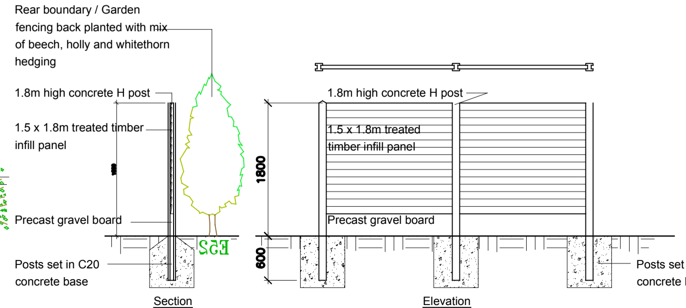
Rear Garden Screen Fence Detail Scale 1:50
