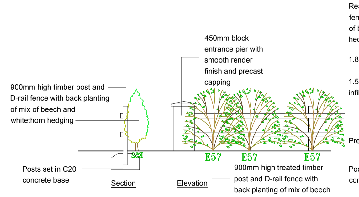
Front Garden Low level Fence Detail Scale 1:50
