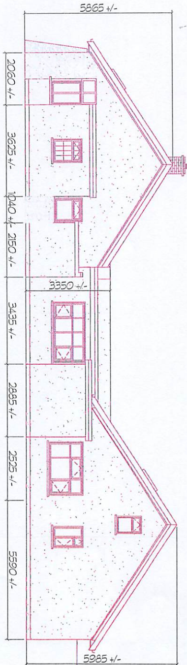
2 EXISTING NORTH REAR ELEVATION 1:100
