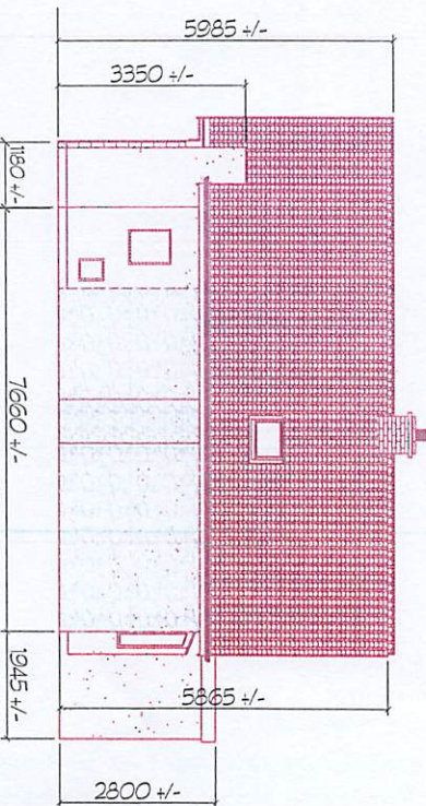
3 EXISTING EAST ELEVATION 1:100
