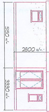
5 EXISTING APT 5 SOUTH ELEVATION 1:100
