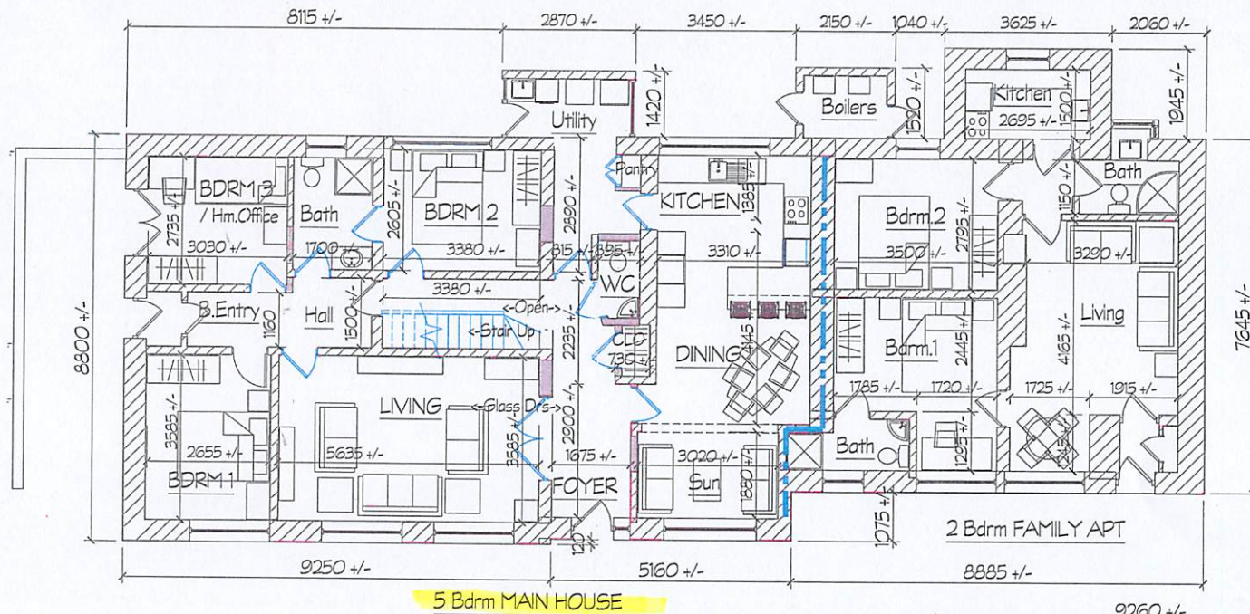
① SCHEME-A GROUND FLOOR LAYOUT 1:100 NOTE NEW (& Rev Swing) DOORS SHOWN BLUE
