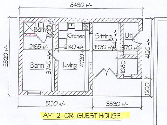
③ DETACHED APT.2 GROUND FLOOR LAYOUT 1:100
