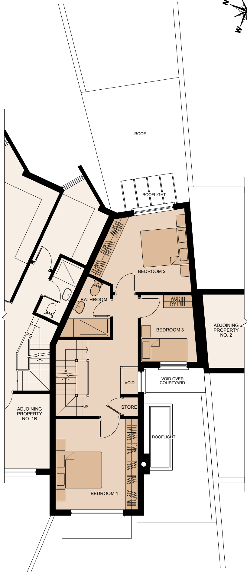
FIRST FLOOR PLAN FLOOR AREA : 52 sqm ( 560 sqft )
