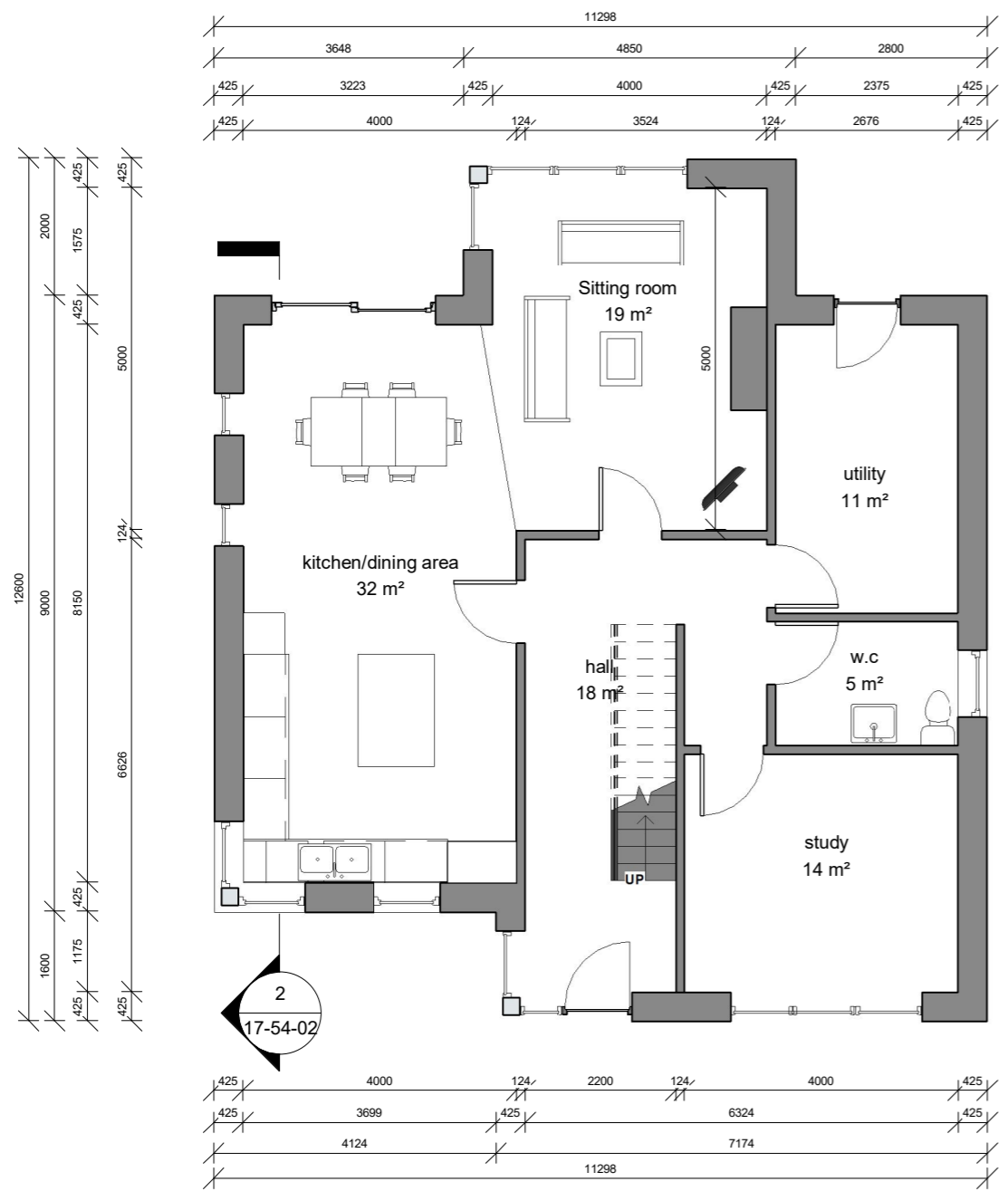
1 LL00 Ground floor plan 1 : 100
