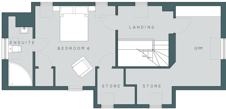
Silver Acre -No. 724 Howth Road Second Floor Plan
