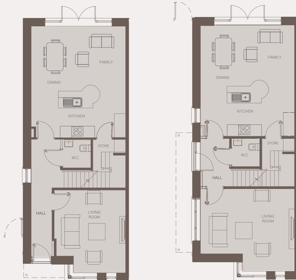
GROUND FLOOR P1 - Front Entrance
