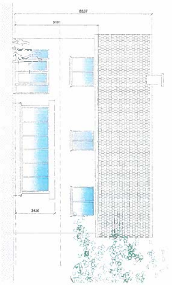
SOUTH ELEVATION (HOUSE TYPE 2)
