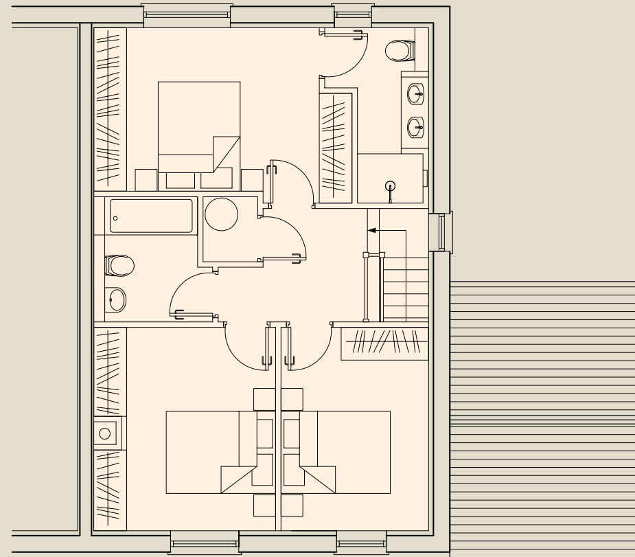
FIRST FLOOR
